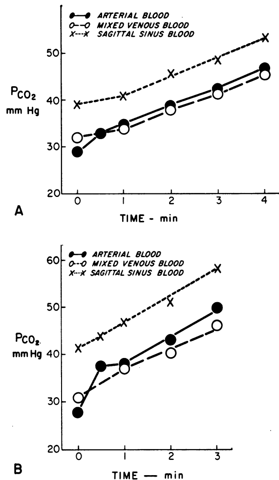
FIGURE 1 Rise of arterial, mixed venous, and cerebral venous (sagittal sinus) PCO_2 during apneic oxygenation (A) and asphyxia (B) in an anesthetized and paralyzed dog. In (A) arterial O_2 saturation was maintained above 98%. In (B) it fell from 94% to 40%. Within 1 min arterial and mixed venous PCO_2 values became nearly equal and thereafter PCO_2 at all three sampling sites rose linearly with respect to time, and at equal rates.
