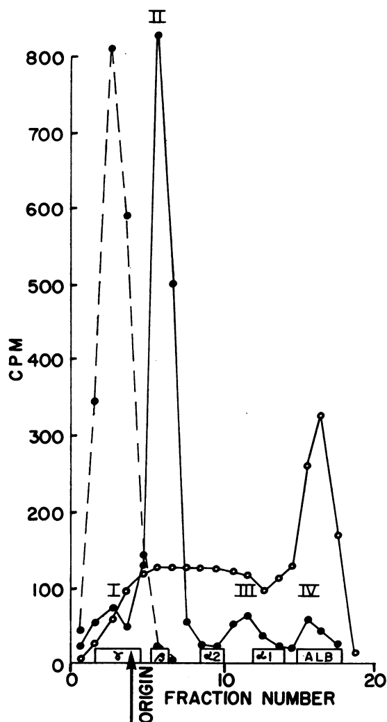
FIGURE 1 The electrophoretic migration of testosterone- ^3\text{H} in buffer, with human serum albumin, and with plasma from a normal male. The anode is on the right. The origin indicates the point of application. Each fraction number is a 0.5 cm portion of the paper cut at right angles to the direction of migration of the proteins, starting 2.25 cm cathodal to the origin. The amount of radioactivity recovered in a single cut is represented by a point in the center of the fraction. The dashed line represents the migration of testosterone- ^3\text{H} in pH 7.4 phosphosaline buffer. The solid line with open circles represents the migration of testosterone- ^3\text{H} when mixed before application with human serum albumin, 5 g/100 ml. The solid line with closed circles represents the migration of testosterone- ^3\text{H} with plasma. I indicates the peak of radioactivity which migrates cathodal to the origin as does testosterone in buffer; II indicates the peak of radioactivity associated with the \beta -globulins; III , that with the inter- \alpha -globulins; and IV , that with albumin. Electrophoresis was carried out at room temperature in Durrum tanks for 20 hr in 0.055 M glycine acetate buffer, pH 8.6, with an applied voltage of 5.3 v/cm.
