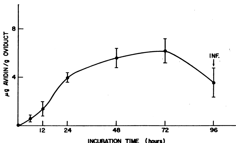
FIGURE 1 In vitro avidin induction curve. Progesterone (5 \mu g) was added at zero time to minced, weighed oviduct in 1 ml of 199 tissue culture medium (N.I.H.) and incubated at 38°C for 96 hr under 95% O 2 -5% CO 2 in a Dubnoff metabolic incubator. Incubation flasks were frozen at the indicated times and assayed for avidin. Each point represents the mean \pm SE of six oviducts analyzed separately. Infection (INF) occasionally occurred at this time point.
