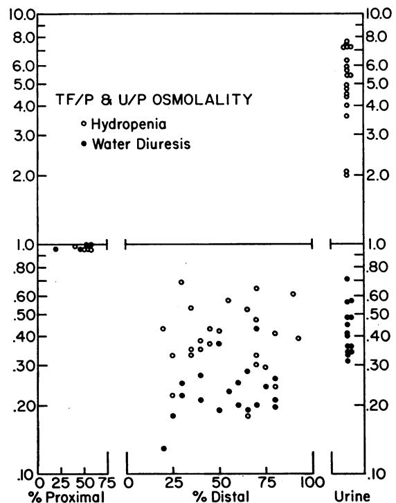
FIG. 1. OSMOLAL TF/P RATIOS FOR PROXIMAL AND DISTAL TUBULAR FLUID OF THE DOG DURING HYDROGENIA OR WATER DIURESIS. TF/P = tubular fluid to plasma; U/P = urine to plasma.
