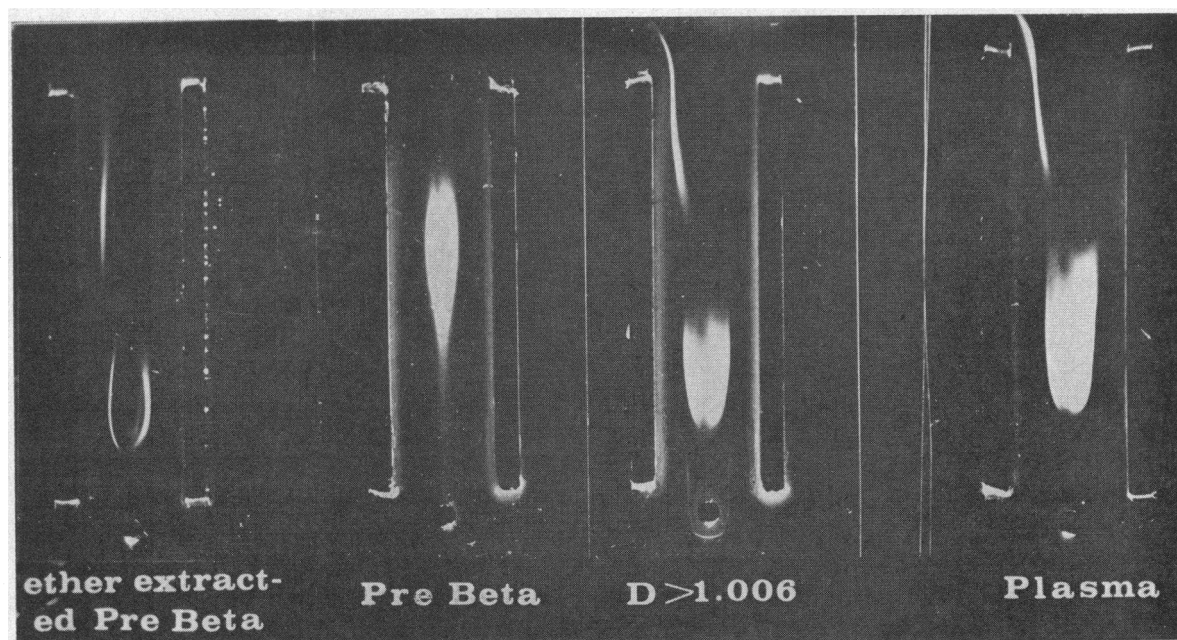
FIG. 7. IMMUNOELECTROPHORESIS ON AGAROSE OF WHOLE PLASMA AND PRE-BETA LIPOPROTEIN BEFORE AND AFTER ETHER DELIPIDATION. Antiserum \text{SL}_A (combined anti-alpha and beta lipoprotein sera) was employed in the left-hand trough and antiserum \text{R}_7 (anti-beta lipoprotein serum) in the right-hand trough. All precipitin bands have been subsequently stained with Oil Red O.
