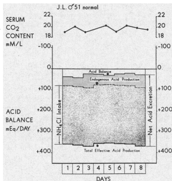
FIG. 1. ACID BALANCE AND SERUM \text{CO}_2 CONTENT IN A NORMAL SUBJECT GIVEN 280 mEq OF \text{NH}_4\text{Cl} DAILY. See text for further details.
