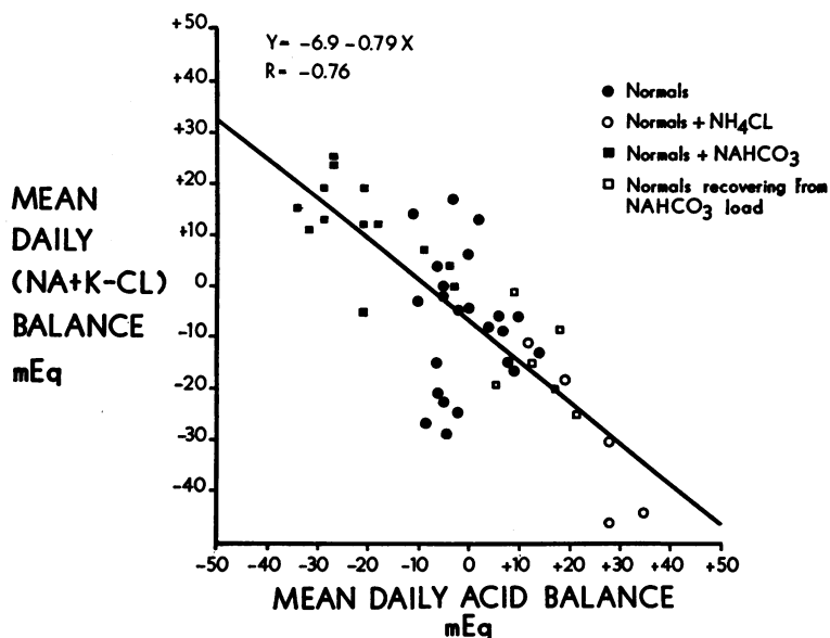
FIG. 3. RELATION BETWEEN MEAN DAILY BALANCE OF (NA + K - CL) AND THE MEAN DAILY ACID BALANCE IN THE 41 STUDIES SUMMARIZED IN TABLE VII AND IN SIX OTHER STUDIES DURING RECOVERY FROM A LOAD OF NAHCO 3 .
