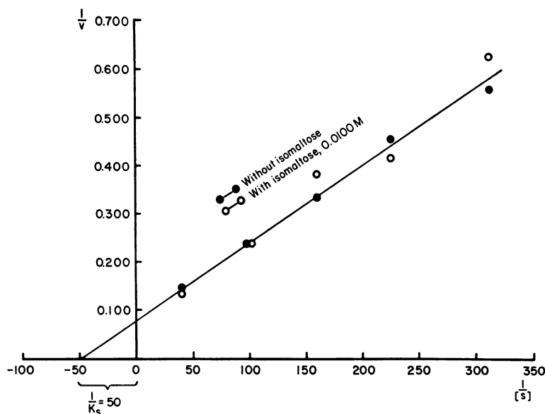
FIG. 3. LINEWEAVER-BURK-DIXON PLOT OF INVERTASE ACTIVITY WITH (0.0100 M) AND WITHOUT ISOMALTOSE. Isomaltose does not inhibit intestinal invertase. v = rate of hydrolysis of sucrose and [s] = concentration of substrate (sucrose) in moles per liter.
