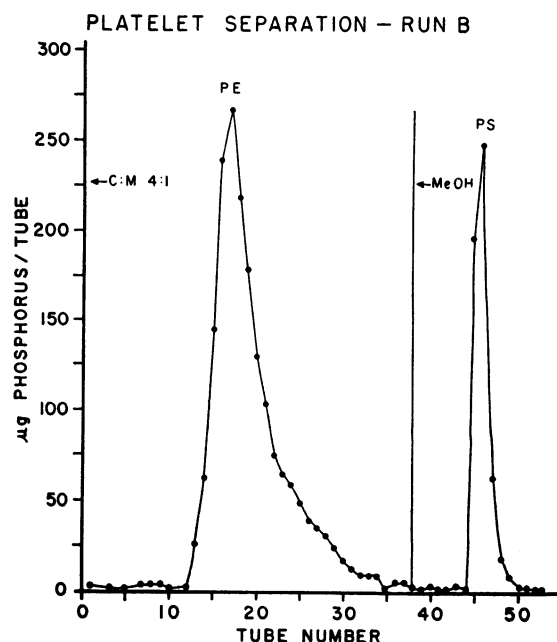
FIG. 3. SEPARATION OF PHOSPHATIDYL ETHANOLAMINE (PE) FROM PHOSPHATIDYL SERINE (PS) ON AN AMMONIATED SILICIC ACID COLUMN. The column was made alkaline by passage of 70 ml ammoniated chloroform: methanol 4:1 before application of PE-PS (3). Consequently PE was eluted first, but PS was retained and recovered later with methanol.
