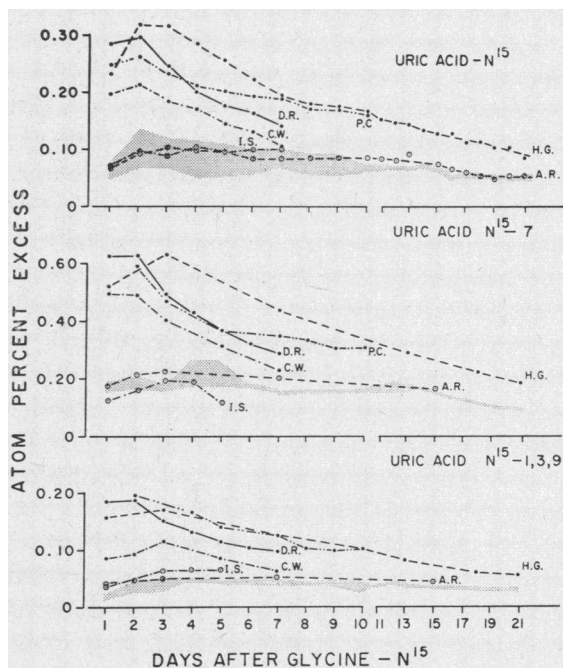
FIG. 2. URIC ACID-N 15 (TOP), URIC ACID N 15 -7 (MIDDLE), AND URIC ACID N 15 -(1+3+9) (BOTTOM), EXPRESSED AS ATOM % EXCESS N 15 , AFTER ADMINISTRATION OF GLYCINE-N 15 TO GOUTY OVEREXCRETORS (SOLID CIRCLES) AND GOUTY NORMAL EXCRETORS (OPEN CIRCLES). Approximate normal range of variation is indicated by shaded area. Note that ordinate for N 15 -7 is drawn to twice the scale of the others.
