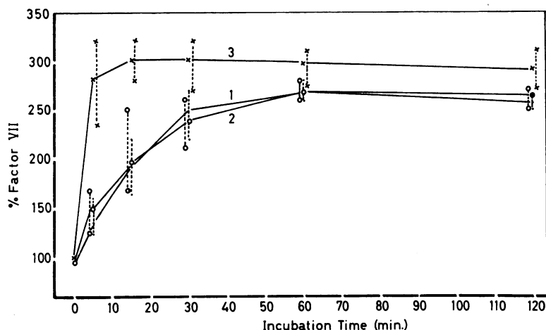
FIG. 1. NORMAL BLOOD—DEVELOPMENT OF INCREASED FACTOR VII ACTIVITY DURING CLOTING WITH ADDED: SALINE, CURVE 1 (—); THROMBIN, CURVE 2 (○—○); AND THROMBOPLASTIN, CURVE 3 (×—×). Five subjects were studied and the range of the results for each of the additives is indicated by broken lines at each incubation time. The curves were constructed by connecting the points representative of the average of the determinations for each incubation time.
