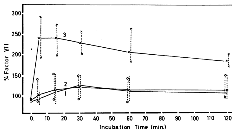
FIG. 3. FACTOR IX DEFICIENT BLOOD—DEVELOPMENT OF INCREASED FACTOR VII ACTIVITY DURING CLOTTING WITH ADDED: SALINE, CURVE 1 (—); THROMBIN, CURVE 2 (○—○); AND THROMBOPLASTIN, CURVE 3 (×—×). Five subjects were studied and the range of the results, for each of the additives, indicated by broken lines at each incubation time. The curves were constructed by connecting the points representative of the average of the determinations for each incubation time.
