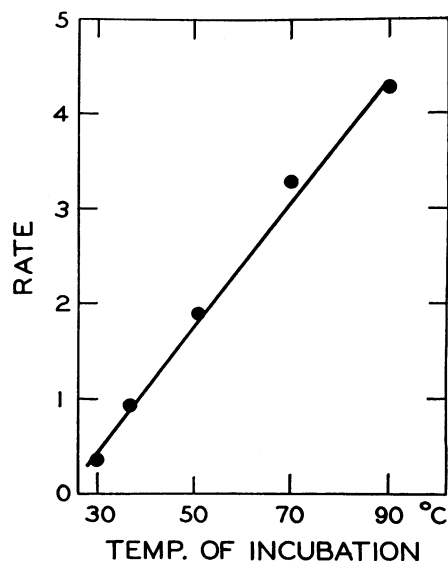
FIG. 2. THE RATE OF ENDOTOXIN INACTIVATION BY PLASMA AT VARIOUS TEMPERATURES OF INCUBATION. Conditions of reaction: resin-treated human plasma 72 per cent, concentration of endotoxin 142 \mu\text{g} per ml, pH 7.3, incubated 10 to 30 minutes. Aliquot tested: 0.14 ml per animal.
