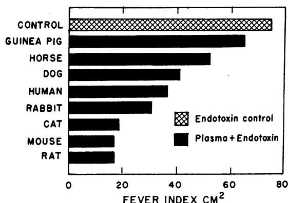
FIG. 7. THE CAPACITY OF PLASMA FROM DIFFERENT SPECIES TO INACTIVATE ENDOTOXIN IN VITRO . Conditions of reaction: citrated plasma 36 per cent, concentration of endotoxin 142 \mu g per ml, pH 7.1 to 7.4, incubated 60 minutes at 37° C. Aliquot tested: 0.14 ml per animal.
