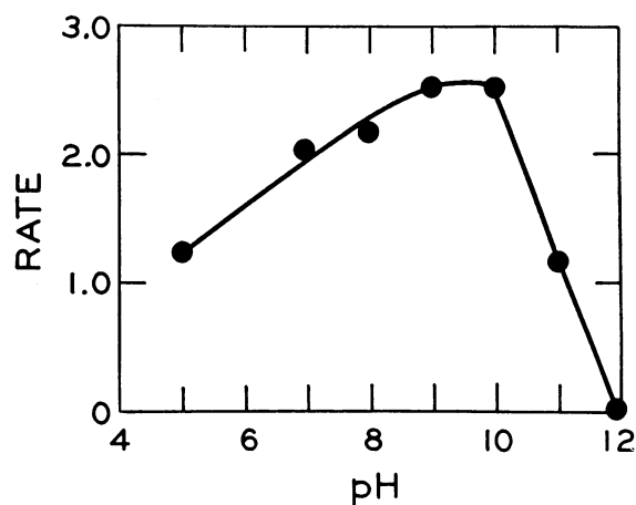
FIG. 5. THE RATE OF ENDOTOXIN INACTIVATION BY PLASMA IN REACTION MIXTURES OF DIFFERENT pH. Conditions of reaction: citrated rabbit plasma 36 per cent, concentration of endotoxin 142 μg per ml, incubated for 15 minutes at 37° C. Aliquot tested: 0.14 ml per animal.
