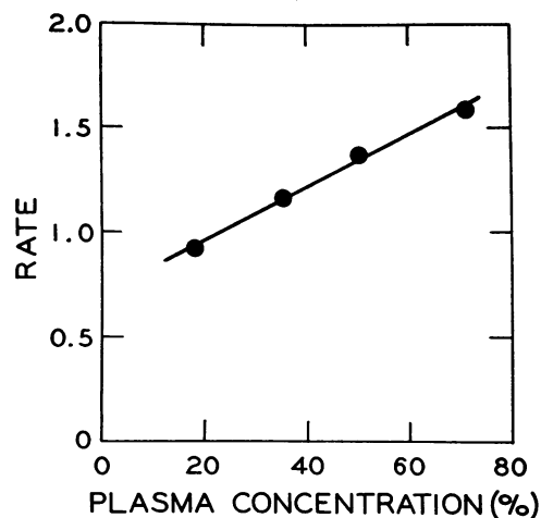
FIG. 4. EFFECT OF THE CONCENTRATION OF PLASMA ON THE RATE OF ENDOTOXIN INACTIVATION. Conditions of reaction: citrated rabbit plasma 18 to 72 per cent, concentration of endotoxin 142 μg per ml, pH 7.6, incubated 30 minutes at 37° C. Aliquot tested: 0.14 ml per animal.
