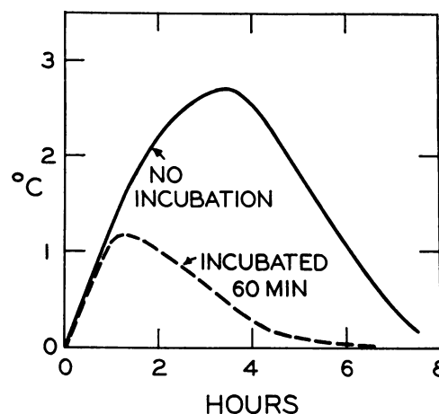
FIG. 1. THE FEBRILE RESPONSE TO EQUAL ALIQUOTS OF A PLASMA-ENDOTOXIN REACTION MIXTURE BEFORE AND AFTER INCUBATION. Conditions of reaction: resin-treated human plasma 80 per cent, concentration of endotoxin 200 \mu\text{g} per ml, pH 7.4, incubated 60 minutes at 37° C. Aliquot tested: 0.10 ml per animal.
