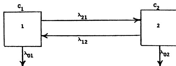
FIG. 2. A TWO-COMPARTMENT SYSTEM MODEL. C_1 = volume of compartment 1 and is equal to pool size of stable thyroxine with plasma as shown in Table I; C_2 = volume of compartment 2; \lambda_{01} and \lambda_{02} = the turnover rates from C_1 and C_2 , respectively; \lambda_{21} and \lambda_{12} = the turnover rates from C_1 into C_2 and from C_2 into C_1 , respectively; \lambda_{11} = \lambda_{01} + \lambda_{21} ; \lambda_{22} = \lambda_{02} + \lambda_{12} .
