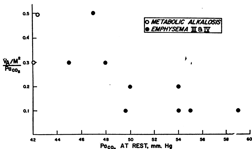
FIG. 3. SENSITIVITY TO THE \text{CO}_2 STIMULUS AS A FUNCTION OF THE DEGREE OF CARBON DIOXIDE RETENTION
