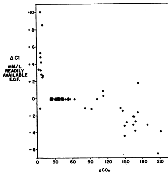
FIG. 4. TRANSFER OF CHLORIDE PER LITER OF READILY AVAILABLE EXTRACELLULAR FLUID, AS A FUNCTION OF ARTERIAL \text{pCO}_2 .
