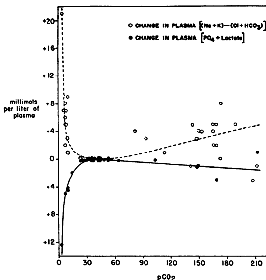
FIG. 5. VARIATIONS IN ANION DEFICIT, AS A FUNCTION OF ARTERIAL \text{pCO}_2 .
