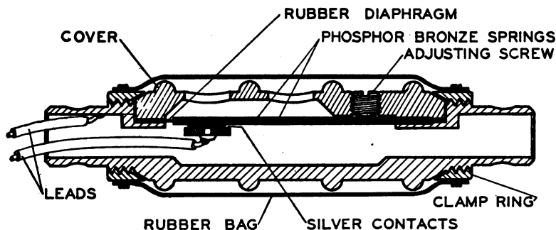
FIG. 2. SCALE DRAWING OF PRESSURE-SENSITIVE CAPSULE Overall length 26 mm.; diameter approximately 5 mm.
