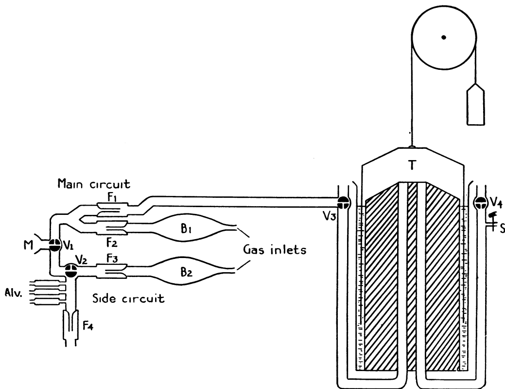
FIG. 2. APPARATUS FOR MEASUREMENT OF NITROGEN EXCRETION
