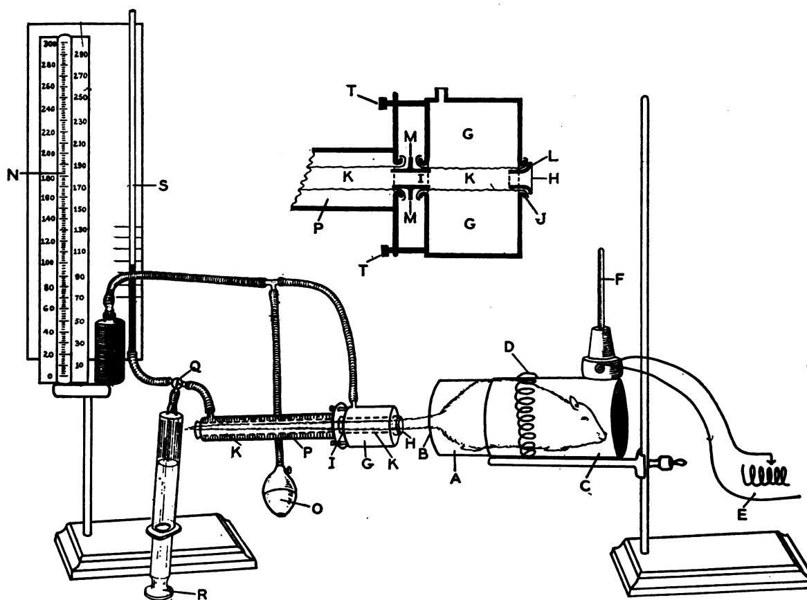
FIG. 1. BLOOD PRESSURE APPARATUS AND RAT HOLDER
