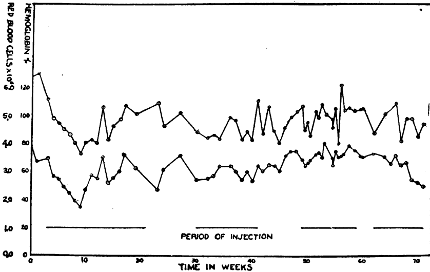
CHART 4. RED BLOOD CORPUSCLES AND HEMOGLOBIN FOLLOWING SUBCUTANEOUS AND INTRAPERITONEAL INJECTION OF WELCH BACILLUS TOXIN Upper graph—red blood cells; lower graph—hemoglobin
