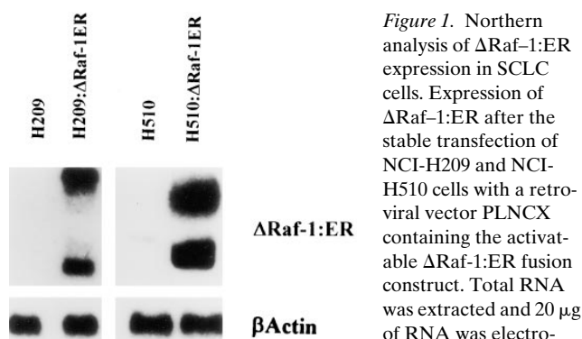
Figure 1. Northern analysis of ΔRaf-1:ER expression in SCLC cells. Expression of ΔRaf-1:ER after the stable transfection of NCI-H209 and NCI-H510 cells with a retroviral vector PLNCX containing the activatable ΔRaf-1:ER fusion construct. Total RNA was extracted and 20 μg of RNA was electrophoresed through a
