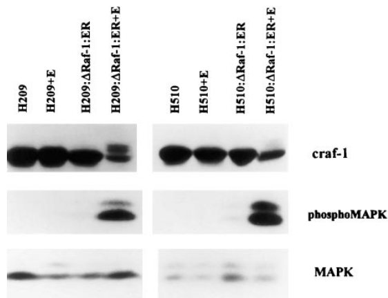
Figure 2. Activation of ΔRaf-1:ER caused the phosphorylation of endogenous c-Raf-1 and MAP kinase in SCLC cells. Lysates from parental SCLC cells, SCLC cells treated with estradiol (+E) for 48 h, NCI-H209-transduced SCLC cells and estradiol-activated ΔRaf-1:ER SCLC cells were immunoblotted with antibodies to Raf-1, phosphorylated MAPK and control MAPK.
