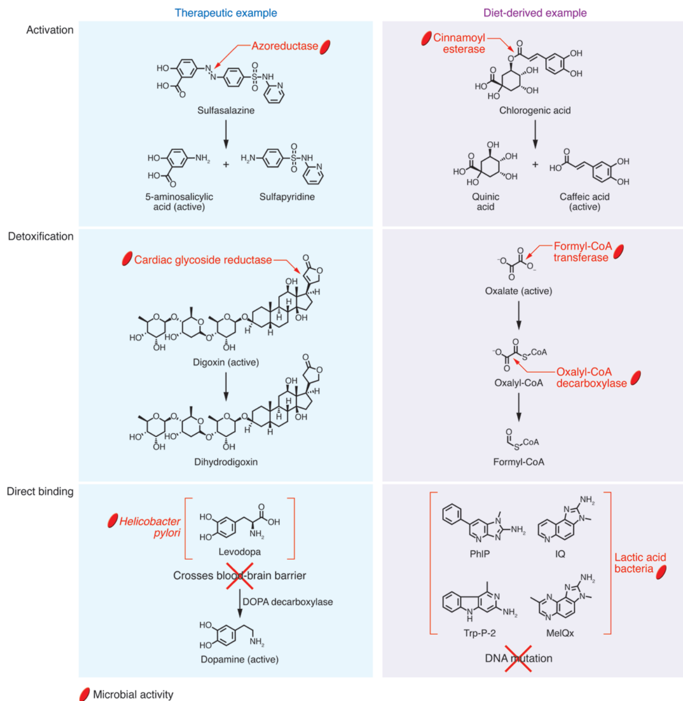
Figure 2. Mechanisms of direct microbial interference with select therapeutic and diet-derived compounds. See article text for detailed descriptions of these interactions.
