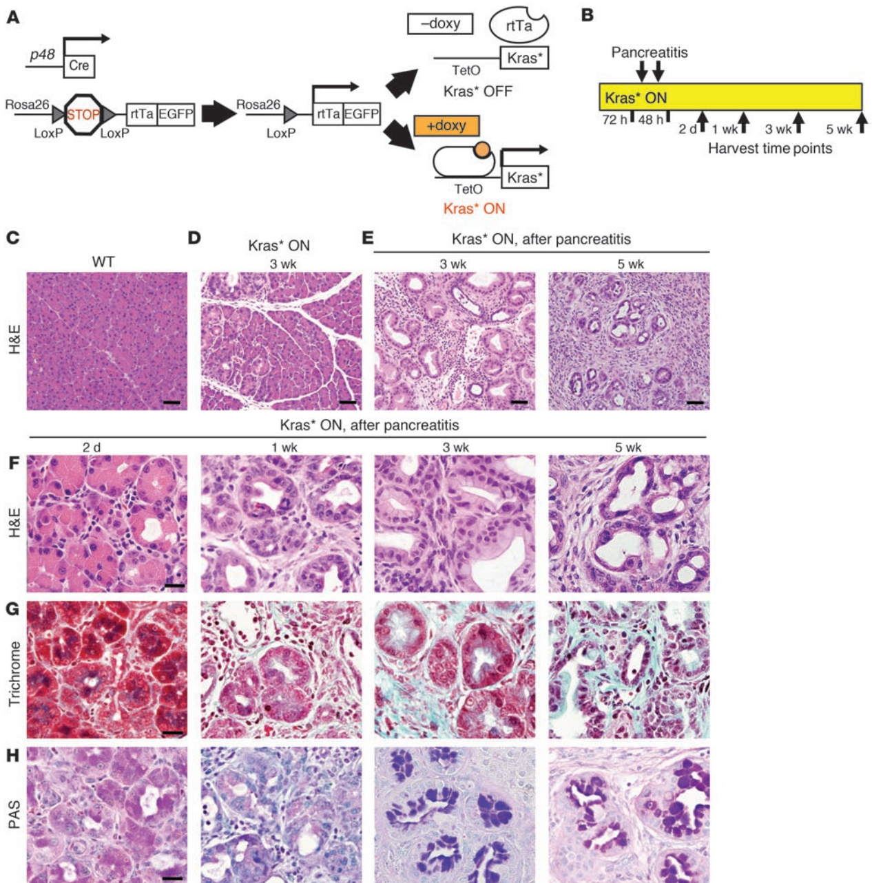
Figure 1 The iKras* mouse model of pancreatic tumorigenesis. (A) Genetic makeup of the iKras* model: p48 - Cre ; R26 - rtTa - IRES - EGFP ; TetO - Kras G12D . (B) Experimental design. Kras* expression was induced with doxy for 72 hours before 2 consecutive days of intraperitoneal cerulein injections to induce pancreatitis and neoplasia. n = 3–5 mice per time point. (C) H&E staining of wild-type murine pancreas. Scale bar: 50 \mu m. (D) H&E staining of iKras* murine pancreas 3 weeks after doxy induction of Kras* . Scale bar: 50 \mu m. (E) H&E staining of iKras* murine pancreas 3 and 5 weeks after induction of Kras* and cerulein injections. Scale bars: 50 \mu m. (F) H&E staining of iKras* murine pancreas 2 days, 1 week, 3 weeks, and 5 weeks after induction of Kras* and cerulein injections. Scale bar: 20 \mu m. (G) Gomori trichrome staining for interstitial collagen 2 days, 1 week, 3 weeks, and 5 weeks after induction of Kras* and cerulein injections. Scale bar: 20 \mu m. (H) PAS staining for mucin accumulation 2 days, 1 week, 3 weeks, and 5 weeks after induction of Kras* and cerulein injections. Scale bar: 20 \mu m.
