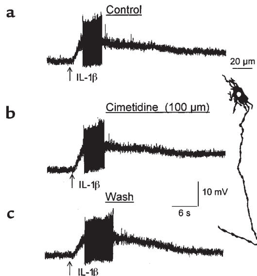
Figure 5 Application of cimetidine did not suppress the depolarizing action and enhanced excitability produced by IL-1 \beta in a neuron with multiple short, dendritic-like processes and a single long process. (a) Depolarization and action potential discharge evoked by a microejection pulse of IL-1 \beta . (b) Responses to IL-1 \beta were unchanged in the presence of cimetidine. (c) Responses to IL-1 \beta after washout of cimetidine. Failure of cimetidine to suppress the response to IL-1 \beta suggested that the action was directly on the neuron rather than due to release of histamine from mast cells.
