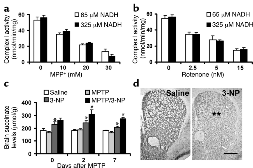
Figure 5 Dose-response study of NADH in complex I activity ( a and b ) and brain levels of succinate ( c ). In mitochondria lysed by freeze-thawing, when the inhibition of complex I activity was titrated with different concentrations of MPP + ( a ) or rotenone ( b ), different amounts of NADH did not produce different responses in complex I activity ( n = 4 per group). ( c ) Levels of succinate were measured in the brains of animals treated with 18 mg/kg/d MPTP or 15 mg/kg 3-NP, or both. Levels of succinate in the group that received D \beta HB (1.6 mmol/kg/d) are significantly increased in the presence of 3-NP. n = 3 –10 per group; * P < 0.05 compared with the control saline group; # P < 0.05 compared with the 3-NP group. ( d ) Histochemical analysis in striatal sections shows that when animals were treated with 3-NP (right panel) at this concentration for 8 days, there was approximately 40% reduction in complex II activity in the striatum compared with that in the group treated with saline (left panel). n = 5 per group; ** P < 0.01 . Scale bar: 500 \mu m.
