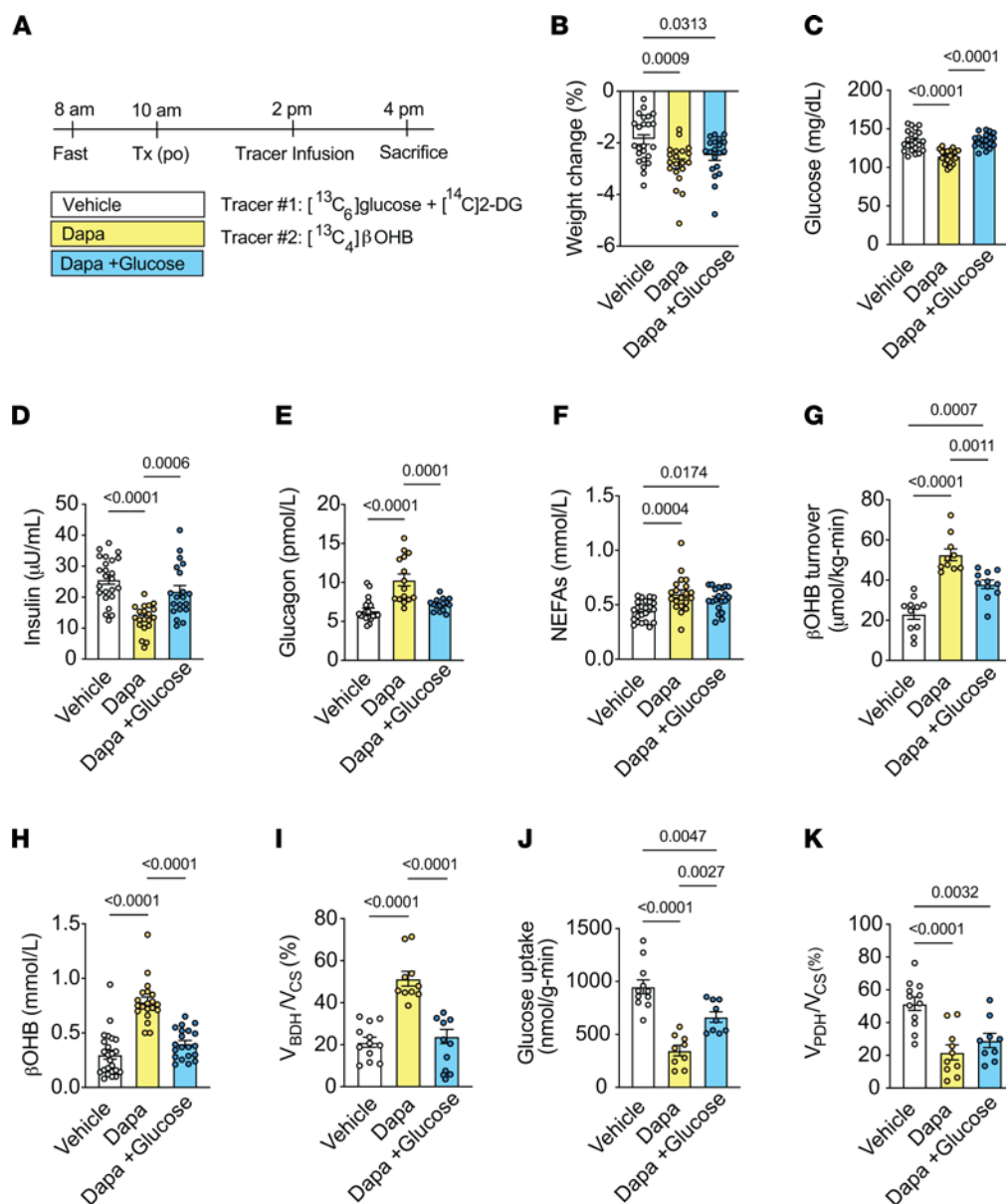
Figure 1. Acute dapagliflozin treatment significantly increases relative rates of βOHB oxidation at the expense of pyruvate oxidation in chow-fed male rats. (A) Outline of study design. Rats were given an intravenous bolus of ^{14}\text{C} [2-DG] during the last 20 minutes of the infusion. (B–K) Weight change (B), plasma glucose (C), plasma insulin (D), plasma glucagon (E), plasma NEFAs (F), whole-body βOHB turnover (G), plasma βOHB (H), relative rates of myocardial βOHB oxidation ( V_{\text{BDH}} ) to total mitochondrial oxidation ( V_{\text{CS}} ) (I), myocardial glucose uptake (J), and relative rates of myocardial pyruvate oxidation ( V_{\text{PDH}} ) to total mitochondrial oxidation ( V_{\text{CS}} ) (K) in chow-fed male rats treated as in A. In panels (B–K), n = 24, 20, 20 (B and D and F); n = 22, 20, 20 (C); n = 24, 19, 19 (E); n = 11, 10, 11 (G); n = 22, 19, 20 (H); n = 12, 10, 11 (I); n = 11, 9, 9 (J); and n = 12, 10, 9 (K). All data are represented as mean \pm SEM. P < 0.05 by 1-way ANOVA with Bonferroni's corrections for multiple comparisons. Dapa, dapagliflozin; Tx, treatment; po, orally.
