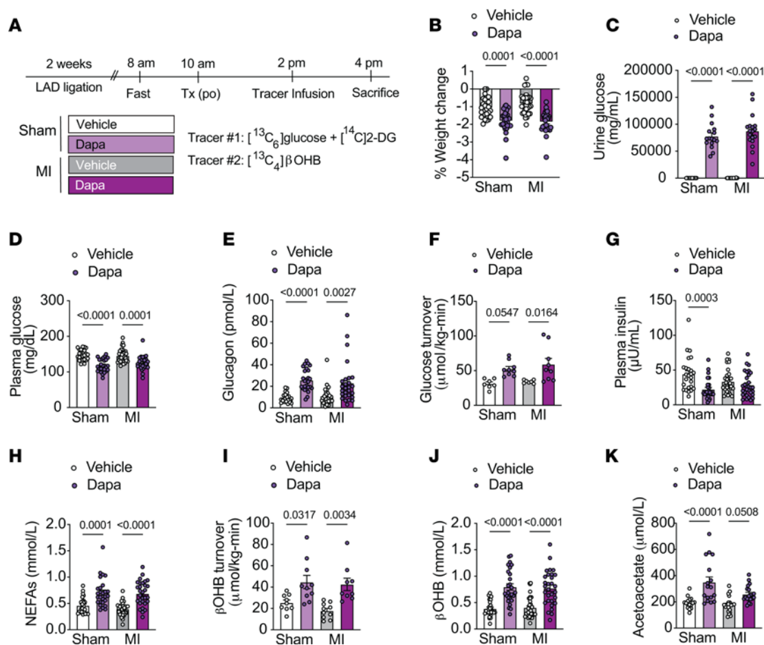
Figure 4. Acute dapagliflozin treatment increases hepatic ketogenesis and plasma ketone levels in sham-surgery and MI rats. (A) Outline of study design. Rats were given an intravenous bolus of [ ^{14}\text{C} ]2-DG during the last 20 minutes of the infusion. (B–K) Weight change (B), urine glucose (C), plasma glucose (D), plasma glucagon (E), whole-body glucose turnover (F), plasma insulin (G), plasma NEFAs (H), whole-body βOHB turnover (I), plasma βOHB (J), and plasma acetoacetate (K) in chow-fed male rats treated as in A. In panels B–K, n = 26, 27, 33, 29 (B); n = 18, 16, 21, 18 (C); n = 24, 26, 32, 29 (D); n = 22, 26, 28, 27 (E); n = 7, 9, 7, 9 (F); n = 25, 27, 32, 30 (G); n = 26, 27, 33, 30 (H and I); n = 9, 10, 10, 9 (I); and n = 16, 17, 21, 19 (K). All data are represented as mean \pm SEM. P < 0.05 by 1-way ANOVA with Bonferroni's corrections for multiple comparisons.
