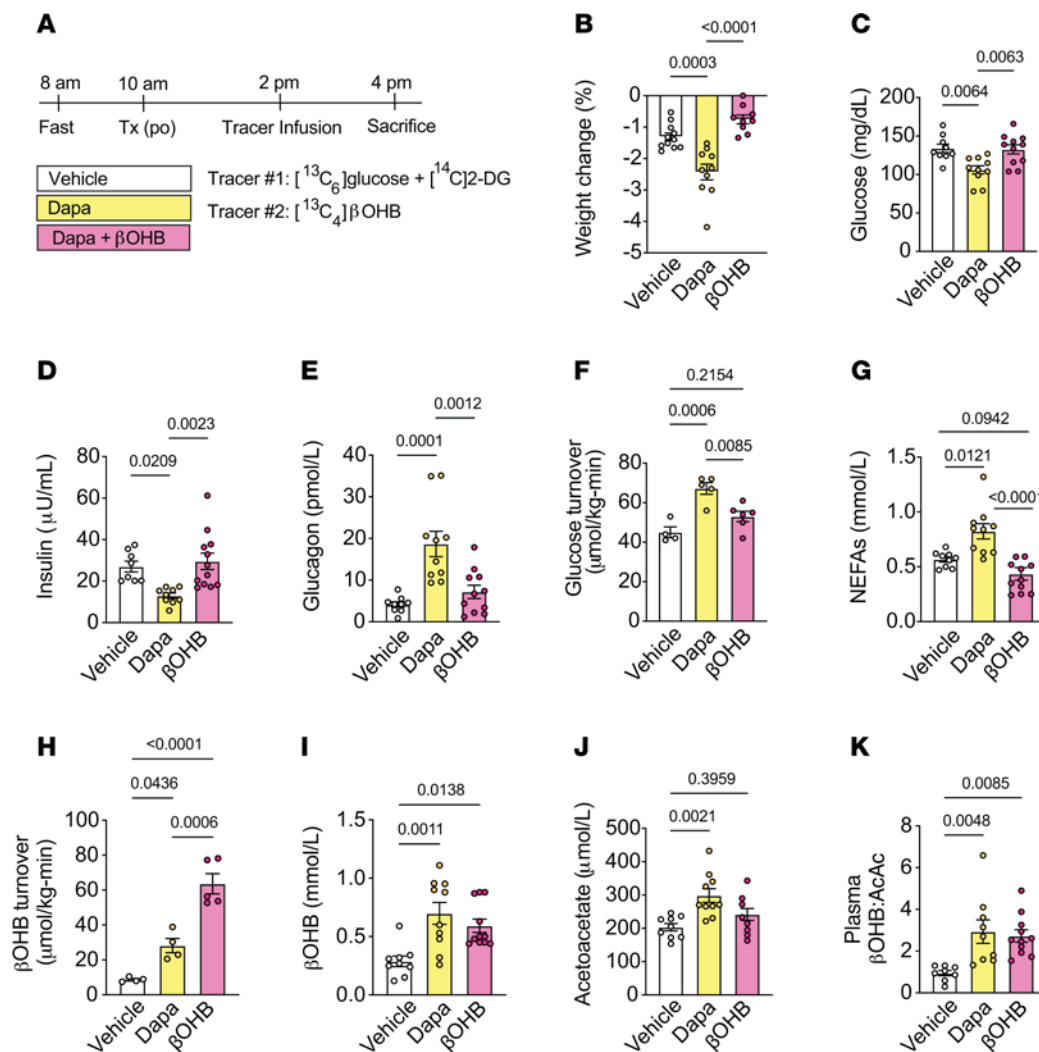
Figure 2. βOHB infusion significantly increases relative rates of βOHB oxidation in chow-fed male rats. (A) Outline of study design. Rats were given an intravenous bolus of ^{14}\text{C} [2-DG] during the last 20 minutes of the infusion. (B–K) Weight change (B), plasma glucose (C), plasma insulin (D), plasma glucagon (E), whole-body glucose turnover (F), plasma NEFAs (G), whole-body βOHB turnover (H), plasma βOHB (I), plasma acetoacetate (J), and plasma βOHB:AcAc in chow-fed male rats treated as in A. In panels (B–K), n = 11, 10, 9 (B); n = 9, 10, 13 (C); n = 8, 9, 12 (D); n = 9, 10, 11 (E, G, and I); n = 4, 5, 6 (F); n = 4, 4, 5 (H); n = 9, 10, 10 (J); and n = 8, 9, 11 (K). All data are represented as mean \pm SEM. P < 0.05 by 1-way ANOVA with Bonferroni's corrections for multiple comparisons.
