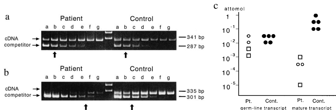
Figure 2. (a) Competitive PCR for the germline C \gamma 2 transcript. Each template contained the same amounts of cDNA from RNA extracted from 7.3 \times 10^3 PBMCs and one of threefold dilutions of germline C \gamma 2 transcript competitor from 1.0 \times 10^{-1} – 1.4 \times 10^{-4} attomole (lanes a–g). Target cDNA and competitor were almost equivalent at 3.3 \times 10^{-2} attomole (lane b) in both the proband and a control, as indicated by arrows . (b) Competitive PCR for mature C \gamma 2 transcript. Each template contained the same amounts of cDNA from RNA extracted from 7.3 \times 10^3 PBMCs and one of tenfold dilutions of mature C \gamma 2 transcript competitor from 1.0 \times 10^1 – 1.0 \times 10^{-5} attomole (lanes a–g). The probands' target cDNAs and competitor were almost equivalent between 1.0 \times 10^{-4} (lane e) and 1.0 \times 10^{-5} attomole (lane f), and those of a control were almost equivalent between 1.0 \times 10^{-1} (lane b) and 1.0 \times 10^{-2} attomole (lane c) as indicated by arrows . (c) The expression levels of germline and mature C \gamma 2 transcripts were plotted logarithmically. ○, patient 1; □, patient 2; ●, controls.
