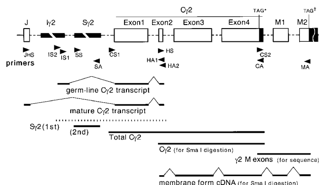
Figure 1. Schematic diagram of PCR strategies. I \gamma 2 and S \gamma 2 regions are indicated by thick bars . Coding exons are indicated by open boxes . 3' Noncoding regions corresponding to secreted and membrane-bound forms of C \gamma 2 cDNAs are indicated by solid boxes . Termination codons of the secreted form (*) and membrane form (†) are marked. Primers are indicated by arrowheads , and their names and sequences are given in Table I. PCR fragments amplified from genomic DNA are indicated by thick lines . The PCR fragment amplified by the first step of nested PCR of S \gamma 2 is indicated by broken thick lines . PCR fragments amplified from cDNA are indicated by fragmented thick lines .
