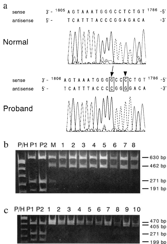
Figure 3. (a) Sequence analysis of the Cγ2 gene (antisense patterns). The proband sequence had a 1790T to C substitution (1790T/C; arrow-head) and a 1793G insertion (1793insG; arrow). (b and c) Sma I-digested PCR products of Cγ2 region from genomic DNA (b) and cDNA for my2HC (c). P/H, size marker; P1 and P2, patients; M, their mother; 1–10, controls. The PCR product from genomic DNA is 1092 bp long and yields the expected 630- and 462-bp fragments (normal) or 630-, 271-, and 191-bp fragments (mutant) after Sma I digestion. The PCR product from cDNA is 875 bp long and yields the expected 470- and 405-bp fragments (normal) or 405-, 271-, and 199-bp fragments (mutant) after Sma I digestion. In case of the cDNA, both 1790T/C and 1793insG are required for Sma I digestion (see a).
