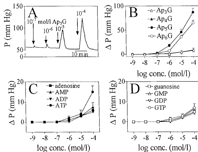
Figure 4. Effects of adenosine(5')oligophospho-(5')guanosines and guanosine(5')oligophospho-(5')guanosines ( \text{Ap}_n\text{G} , \text{Gp}_n\text{G} , n = 3-6 ) as well as of potential degradation products on perfusion pressure in an isolated perfused rat kidney. Data are means \pm SD. (A) Changes in perfusion pressure P (ordinate) after bolus injections of 100 \mu\text{l} physiological salt solution containing the indicated concentrations of \text{Ap}_5\text{G} . (B) Concentration-response curves showing the changes in perfusion pressure ( \Delta P ) after bolus injections of \text{Ap}_n\text{Gs} as described in A. (C) Concentration-response curves showing the changes in perfusion pressure ( \Delta P ) after bolus injections of adenosine, AMP, ADP, and ATP as described in A. (D) Concentration-response curves showing the changes in perfusion pressure ( \Delta P ) after bolus injections of guanosine, GMP, GDP, and GTP as described in A.
