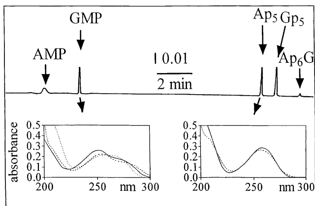
Figure 3. Anion exchange chromatography of the enzymatic cleavage products after incubation of the fraction labeled \text{Ap}_6\text{G} in Fig. 1 C with the 5'-nucleotide hydrolase. The inserts show the UV spectra of the fractions indicated by the arrows (solid line, pH 6.4 [water], dashed lines, pH 2 [0.01 M HCl], dotted lines, pH 11 [10 mM NaOH]). The spectra correspond to those of adenosine and guanosine. The peaks labeled AMP and \text{Gp}_5 showed UV spectra identical with those of \text{Ap}_5 and GMP, respectively.
