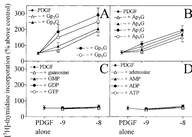
Figure 5. [^3\text{H}] Thymidine incorporation rate (ordinate) in % above control in VSMCs incubated with various concentrations of dinucleoside polyphosphates (A, \text{Gp}_n\text{G} ; B, \text{Ap}_n\text{G} ) and of potential degradation products (C and D) with 5 ng/ml PDGF. Growth stimulation with 5 ng/ml PDGF alone was plotted for comparison. Abscissae: log of concentration in M.
