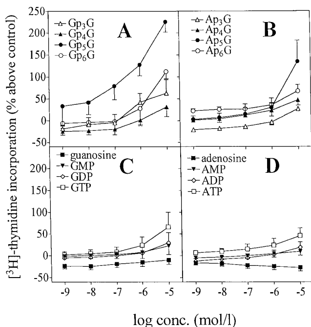
Figure 6. [^3\text{H}] Thymidine incorporation rate (ordinate) in % above control in VSMCs incubated with various concentrations of dinucleoside polyphosphates (A, \text{Gp}_n\text{G} ; B, \text{Ap}_n\text{G} ) and of potential degradation products (C and D) Abscissae: log of concentration in M.
