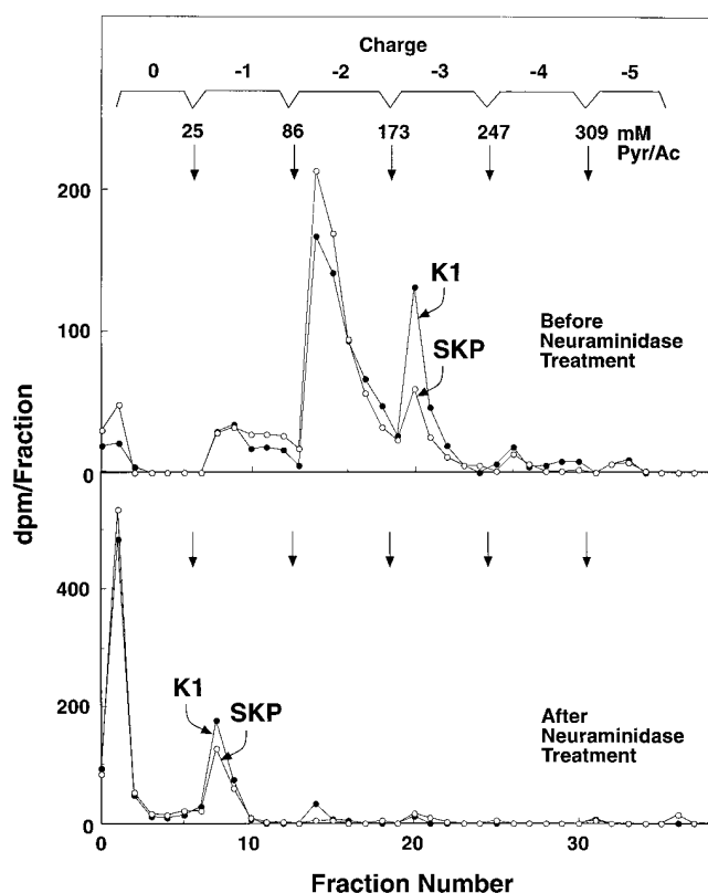
Figure 2. QAE-Sephadex column chromatography of 3 H-GlcN-glycopeptides from CD44 derived from CHO-K1 and -SKP cells before and after treatment with neuraminidase. (Top) The 3 H-GlcN-glycopeptides were applied to a column of QAE-Sephadex in 2 mM pyridyl/acetate (pH 5.5), as described in Methods, and bound glycopeptides were eluted with a step gradient of pyridyl/acetate, as indicated in the top panel. Glycopeptides with increasing negative charges, i.e., degree of sialylation, are eluted as shown. (Bottom) The 3 H-GlcN-glycopeptides were treated with neuraminidase, as described in Methods, and the treated glycopeptides were analyzed by chromatography on QAE-Sephadex. The resultant neutral glycopeptides are not bound by the column, whereas free 3 H-sialic acid released by the neuraminidase is eluted with 25 mM pyridyl/acetate.
