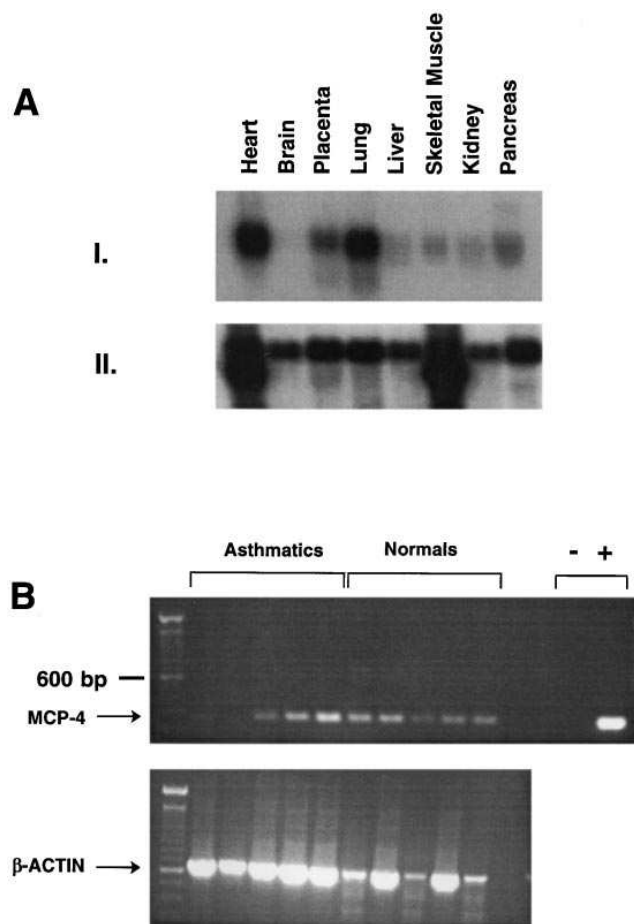
Figure 7. (A) Northern blot analysis of poly(A) ^{+} RNA isolated from several human tissues. (I) Autoradiography of MCP-4 mRNA expression. (II) \beta -Actin mRNA expression from the same blot, after removal of MCP-4 specific probe, showing integrity of RNA and equal loading of lanes. (B) Detection of mRNA for MCP-4 in BAL cells. MCP-4 mRNA was detected by RT-PCR in samples from five BAL cell preparations from unchallenged normal donors and five preparations from mild, unchallenged asthmatic patients. – is the no-template negative control; + is Bluescript plasmid containing MCP-4 coding region used as a positive control. Total RNA was reverse-transcribed and amplified by PCR using MCP-4 (top) and \beta -actin (bottom) specific primers.
