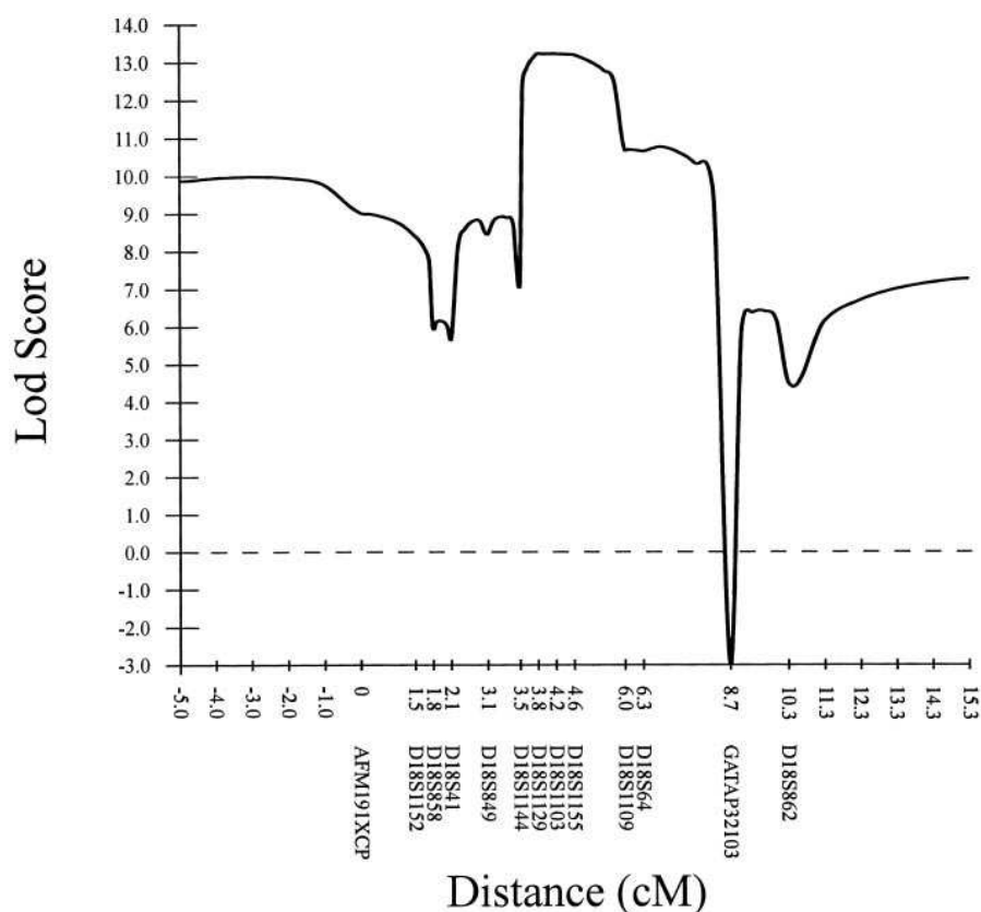
Figure 4. Multipoint linkage analysis of combined Factors V and VIII deficiency. Multipoint linkage analysis was performed using the 13 markers shown on the abscissa with MAPMAKER/HOMOZ. The best distances and order between the markers was determined using MULTIMAP. The markers are shown centromere ( left ) to telomere ( right ). The dotted horizontal line within the plot indicates a LOD score of 0. For marker GATAP32103, the extension to -3.00 represents a point where the LOD score reached -\infty . MAPMAKER/HOMOZ analysis using all 13 markers in the region yielded a maximum LOD score of 13.22 at D18S1129.
