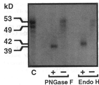
Figure 7. Endoglycosidase digestion of \alpha -GalNAc transiently expressed in COS-1 cells. At 72 h after transfection, \alpha -GalNAc was labeled for 1 h with [ ^{35} S]-methionine and immunoprecipitated. C represents untreated \alpha -GalNAc enzyme; the other samples were treated with either PNGase F or Endo H.
