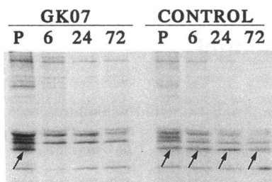
Figure 1. Pulse-chase experiments of fibroblasts. Fibroblasts from patient GK07 and a control individual were pulse labeled with Tran 35 S-label (ICN Biomedicals, Inc., Costa Mesa, CA) for 1 h and were chased for 6, 24, and 72 h. Cell extracts were
