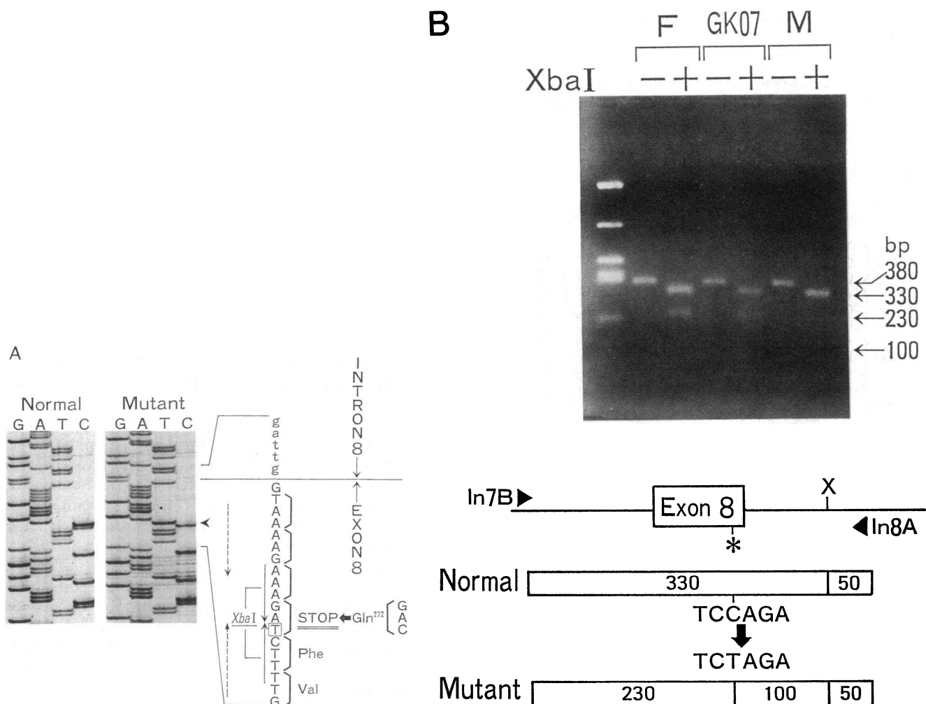
Figure 5. Identification of Q272STOP mutation in the exon 8 sequence. Genomic sequences around exon 8 were amplified with primers In 7B and In 8A. A shows the partial nucleotide sequence around the 5' splice site of intron 8. A C to T mutation (Q272STOP) was identified (arrowhead). This mutation creates an XbaI site. Arrows show palindromic sequences enhanced by the mutation. B demonstrates familial analysis with XbaI digestion. Fragments from the father (lane F) and GK07 were partially digested to 230- and 100-bp fragments, hence they are probably heterozygotes of Q272STOP mutation.
