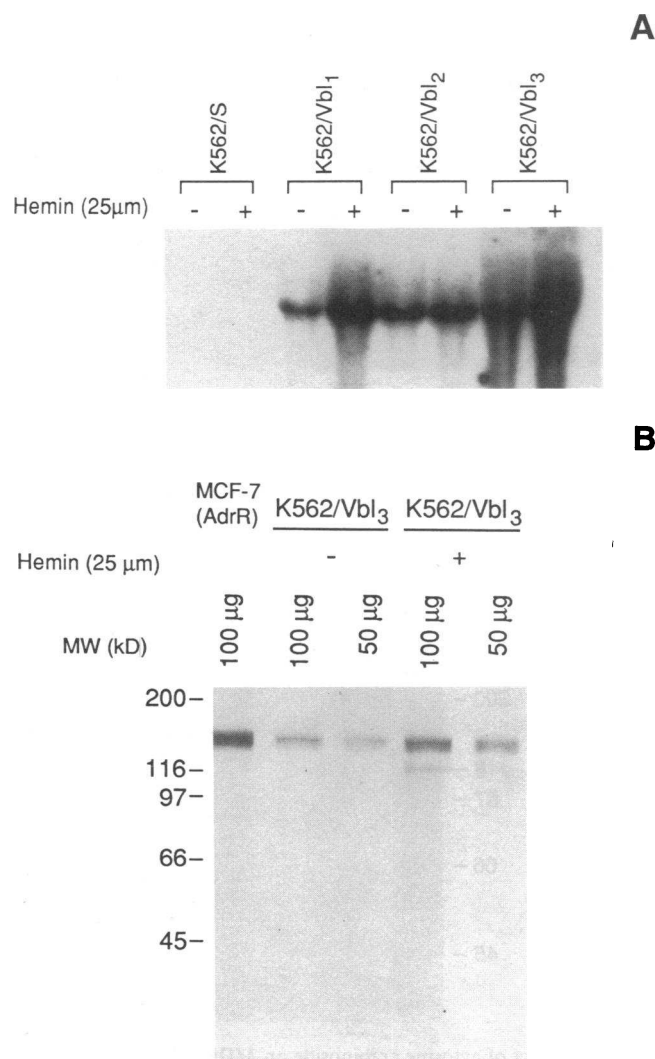
Figure 6. Effect of hemin on MDR1 gene expression in sensitive and resistant K562 cells. (A) MDR1 mRNA: After exposure of sensitive and resistant K562 cells to 25 \mu M hemin for 4 d, RNA was prepared as described in Methods. 20 \mu g of RNA was electrophoresed in 1% agarose/7% formaldehyde gels then transferred to nitrocellulose. Blots were probed using a 4.1-kb MDR1 cDNA insert prepared from the pHaMDR1/A retroviral vector. (B) P-glycoprotein. K562/Vbl 3 cells were exposed to 25 \mu M hemin for 4 d. Membranes were prepared as described in Methods. Proteins were solubilized and electrophoresed on 7.5% SDS gels, transferred to nitrocellulose and probed with the C219 antibody. MCF-7/AdrR cells were used as positive controls.
