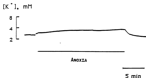
Figure 3. Change in extracellular K^+ concentration ( K_o^+ ) during anoxia. K_o^+ was measured using double-barreled microelectrodes. Anoxia (20 min) induced only a modest increase in K_o^+ (1–2 mM).
