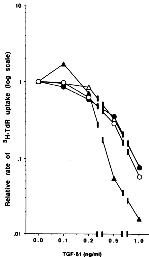
Figure 6. Attenuation of TGF- \beta 1 effect on endothelial cell [ ^3 H]TdR uptake by cysteine. Cystine and TGF- \beta 1 were added at t = 0 h and [ ^3 H]TdR uptake was measured at 120–121 h. Cystine: (▲) none; (Δ) 0.2 mM; (●) 0.5 mM; and (○) 1.0 mM. Cultures done as noted in Methods.
