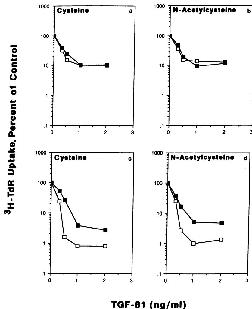
Figure 4. Influence of cysteine and N -acetylcysteine on [ ^3\text{H} ]TdR uptake inhibition by TGF- \beta 1. (□) no cysteine or N -acetylcysteine; (■) + 2 mM cysteine ( a and c ), or 2 mM N -acetylcysteine ( b and d ). [ ^3\text{H} ]TdR uptake was carried out at 72–73 h for ( a and b ) and at 96–97 h for ( c and d ). Other details are in Methods.
