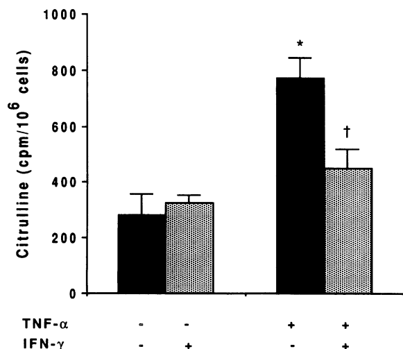
Figure 2. Effect of IFN- \gamma on L-[ 14 C]arginine to L-[ 14 C]citrulline conversion in BAEC. L-[ 14 C]arginine ( 3 \times 10^5 cpm/ml) was added for 3 h to BAEC grown in six-well plates. Following extraction with 1 ml of ice-cold 15% TCA, L-[ 14 C]citrulline in each well was determined by quantitative cation-exchange chromatography. Columns represent L-[ 14 C]-citrulline formation in vehicle (solid bars) or IFN- \gamma -treated BAEC (200 U/ml, 24 h) (gray bars) in the presence or absence of TNF- \alpha (100 ng/ml, 24 h). Each point represents means \pm SE of three experiments, triplicate determinations. * P < 0.05 vs. control. † P < 0.05 vs. TNF- \alpha -treated BAEC in the absence of IFN- \gamma .
