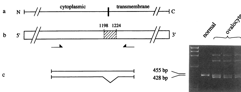
455-bp band represents the normal allele and the smaller 428-bp band represents the mutant allele. Two higher molecular weight bands seen in ovalocytes represent heteroduplexes. Mol wt marker is HaeIII-digested \Phi X174 DNA.
