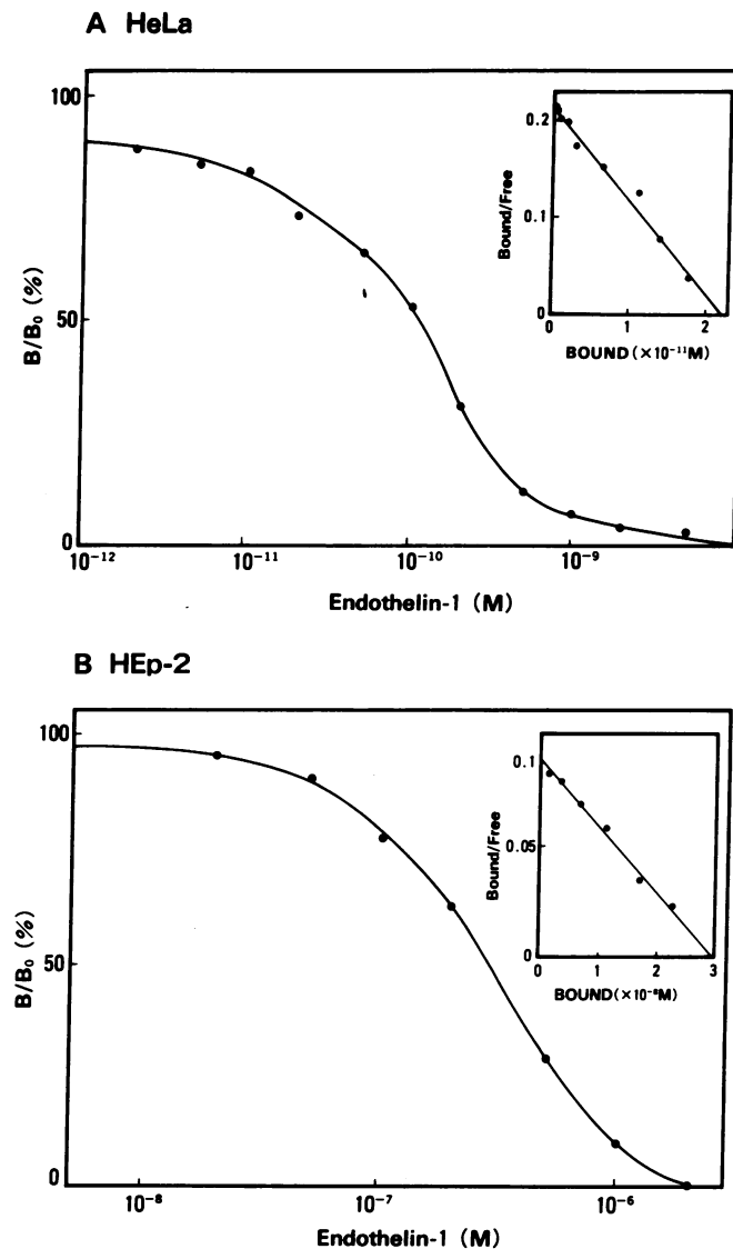
Figure 4. Competitive binding of ^{125} I-ET-1 to cultured HeLa (A) and HEP-2 (B) cells by unlabeled ET-1. Each point is the mean of duplicate determinations. Specific bindings of HeLa and HEP-2 cells were 93 and 79% of total bindings, respectively, after 2 h incubation at 37°C. (Inset) Scatchard analysis of binding data.
