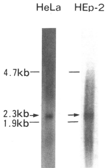
Figure 3. Northern blot analysis of HeLa and HEP-2 cell mRNA. Poly(A) + RNA (10 \mu g) was hybridized with human prepro-ET-1 cDNA as a probe. A single band with a size of 2.3 kb was observed in both tumor cells. Size markers in kilobases are indicated on the left.
