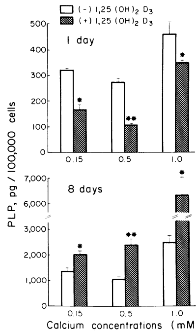
Figure 6. Effect of calcium and 1,25(OH) 2 D 3 on PLP secretion. Normal human keratinocytes were incubated in KBM and increasing calcium concentrations without (open bars) or with (hatched bars) 1,25(OH) 2 D 3 (10 -8 M) for 1 or 8 d. PLP was measured by radioimmunoassay as described in Methods. Each bar is the mean ± SEM of triplicate determinations. The asterisks indicate significant differences in PLP concentrations from incubations at the same calcium concentration but without 1,25(OH) 2 D 3 at P < 0.005 (*) and P < 0.001 (**). The results are representative of three separate experiments.
