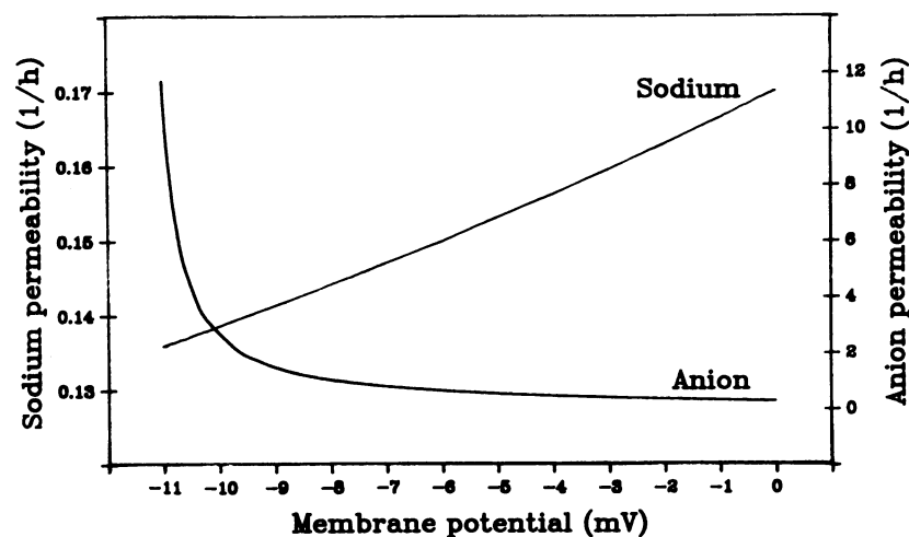
Figure 3. Relation between membrane potential and \text{Na}^+ and \text{Cl}^- (anion) electrodiffusional permeabilities in a reticulocyte model with potential-driven \text{Cl}^- ( \text{A}^- ) entry (option 1). In this option, the two equations for the electrodiffusional \text{Na}^+ and anion fluxes ( \phi_{\text{Na}}^G and \phi_{\text{A}}^G ) link the three unknowns required for the computation of the reference state, membrane potential, and the diffusional permeabilities of \text{Na}^+ and anion ( E , P_{\text{Na}}^G , and P_{\text{A}}^G ; see Appendix). The computing strategy sets the E and derives P_{\text{Na}}^G and P_{\text{A}}^G . The diffusional \text{Na}^+ permeability in all reticulocyte model options exceeds that of mature RBCs by at least two orders of magnitude ( \approx 0.15 \text{ h}^{-1} compared with \approx 0.0015 \text{ h}^{-1} [25]).
