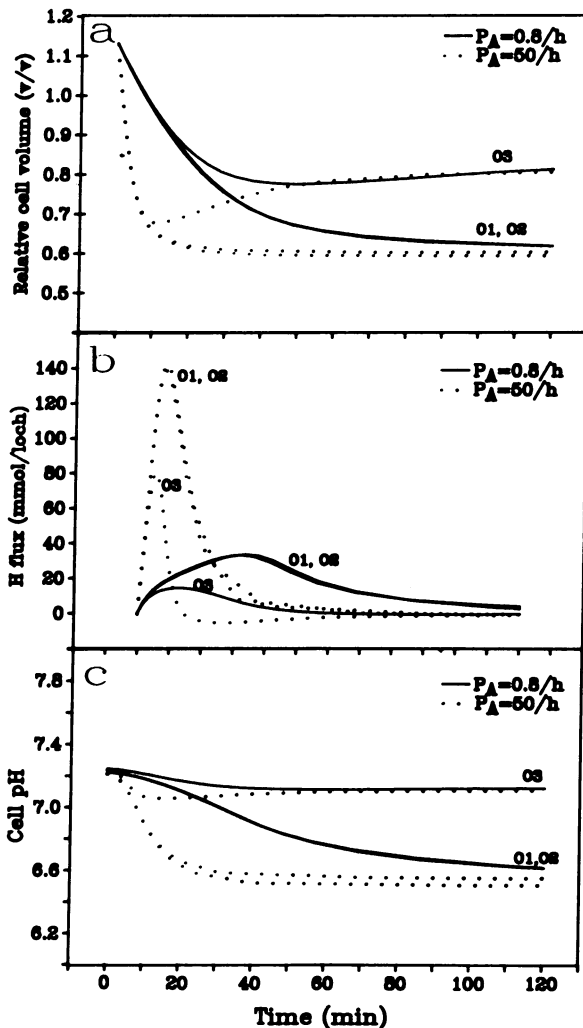
Figure 7. Predicted effects of a sustained increase in \text{K}^+ permeabilization, with or without a concomitant increase in \text{Cl}^- ( \text{A}^- ) permeabilization, on variables of the reticulocyte model, options 1–3. Variables reported are shown in plot ordinates. Anion permeabilities ( P_A ) are shown.
