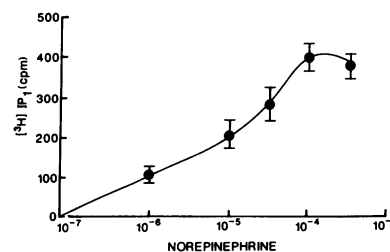
Figure 6. Dose-dependent stimulation of [ ^3 H]IP _1 formation by norepinephrine. Myocytes labeled with [ ^3 H]myoinositol were incubated at various concentrations of norepinephrine for 10 min. n = 2 or 3 separate determinations at each point.
