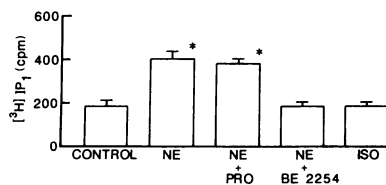
Figure 5. Receptor specificity of norepinephrine stimulated phosphoinositol turnover. [ ^3 H]myoinositol-labeled myocytes were incubated for 40 min
