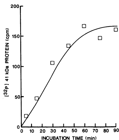
Figure 2. Incorporation of pertussis toxin specific counts into membranes prepared from control hearts as a function of time. Incorporation of [ ^{32} P]NAD was maximal at 60 min. Gels were counted by AMBIS radioanalytic scanner.
