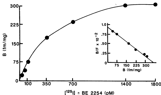
Figure 1. Saturation isotherm and Scatchard analysis of [ ^{125} I]±BE 2254 binding to membranes prepared from the left ventricle of infarcted hearts. Membranes were incubated with increasing concentrations of [ ^{125} I]±BE 2254, and specific binding determined. (Inset) Scatchard transformation of saturation isotherm data.
