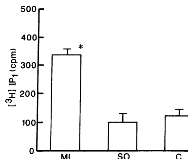
Figure 7. Norepinephrine stimulated [ ^3 H]IP _1 formation in myocytes isolated from infarcted, sham-operated, and nonoperated control rat hearts. Rats were labeled with [ ^3 H]myoinositol and incubated with 100 \mu M norepinephrine. *A value that is statistically and significantly different; P < 0.05 ; n = 4 in all determinations.
