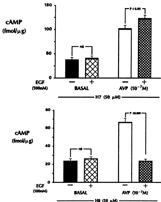
Figure 6. Effect of protein kinase inhibitors on EGF-inhibition of AC. Cells are exposed to H7 (top, n = 6 ) or H8 (bottom, n = 5 ) for 5 min before and during incubation without or with EGF. H7 prevents inhibition by EGF; H8 does not.
