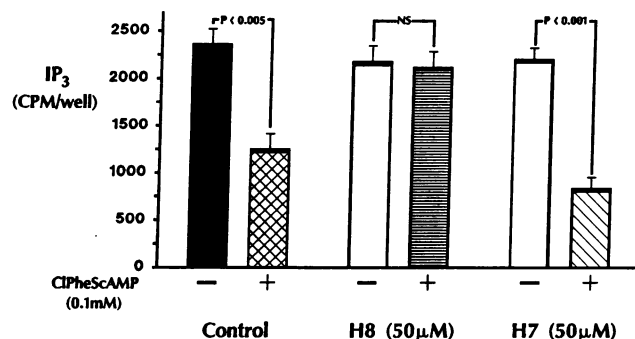
Figure 3. Effect of protein kinase inhibitors on cAMP inhibition of PLC ( n = 4 ). Cells are exposed to H7 or H8 for 5 min before and during exposure to CIPheScAMP. Pretreatment with H8, but not with H7, prevents inhibition by cAMP.
