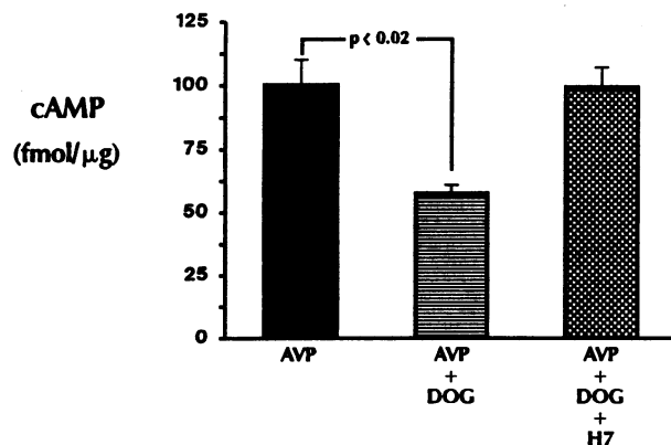
Figure 7. Effect of DOG on AVP-stimulated cAMP generation ( n = 3 ). DOG (100 nM) was added simultaneously with 10 -7 M AVP; H7 was present for 5 min before incubation with DOG. DOG inhibited AVP-stimulated cAMP generation; inhibition was not observed in the presence of H7.
