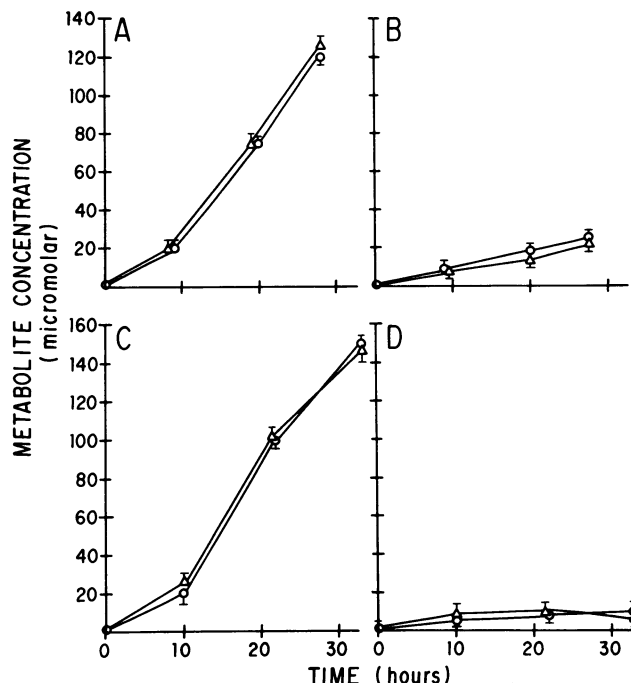
Figure 4. Production of citrulline, nitrite and nitrate by macrophages. CM (A, B, and C) or RM (D) were cultured in DME containing 100 \text{ ng/ml} endotoxin and 500 \text{ nCi/ml} U- [^{14}\text{C}] arginine. Medium in B contained 50 \mu\text{M} N^G -monomethyl-L-arginine. At the times shown supernate medium was collected for measurement of the total \text{NO}_2^- + \text{NO}_3^- (triangles) and radioactive citrulline (circles). Values are means \pm SEM of triplicate cultures per time point. Macrophage protein per well was 0.060 \text{ mg} , (A); 0.057 \text{ mg} , (B); 0.075 \text{ mg} , (C); and 0.055 \text{ mg} , (D).
