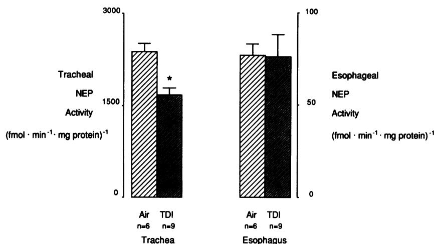
Figure 4. Mean ( \pm SEM) values for NEP activity in the trachea (left columns) and esophagus (right columns) of animals exposed to air or to TDI. *Significantly less than value for animals exposed to air, P < 0.002 .
