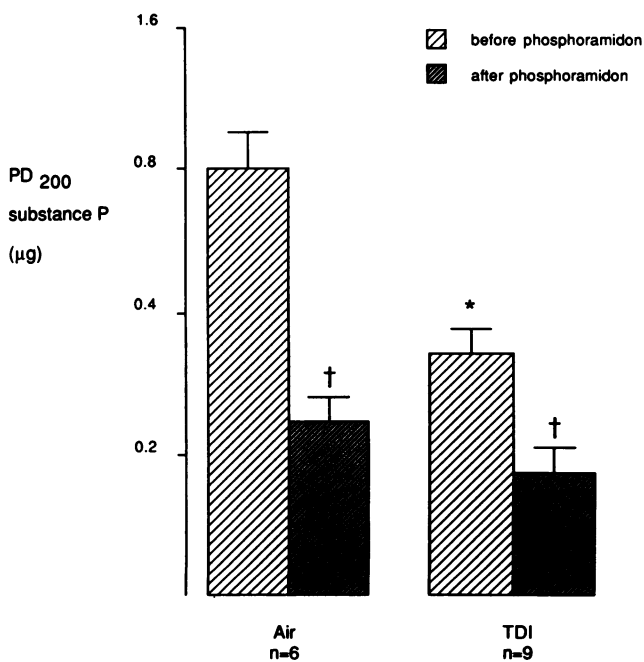
Figure 2. Mean ( \pm GSEM) values for the dose of substance P calculated to cause a 200% increase in pulmonary resistance above baseline ( PD_{200} substance P) before and after phosphoramidon in animals studied after exposure to air or to TDI. * PD_{200} substance P significantly less than PD_{200} after air exposure and before phosphoramidon, P < 0.001 . †Significantly lower than value before phosphoramidon, P < 0.01 .
