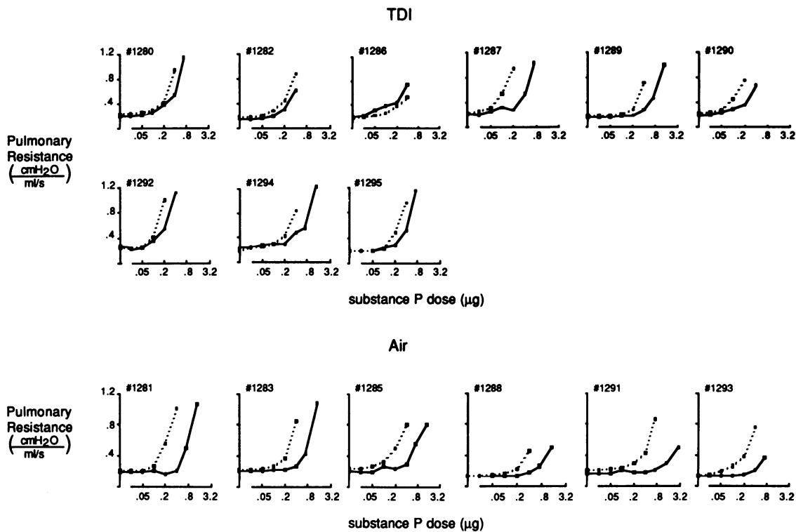
Figure 1. Individual dose-response curves plotting the increases in pulmonary resistance caused by intravenous administration of increasing doses of substance P before (solid lines) and after (dotted lines) intravenous administration of phosphoramidon (0.5 mg). Upper panel shows curves in animals exposed to TDI and lower panel shows curves in animals exposed to filtered air.
