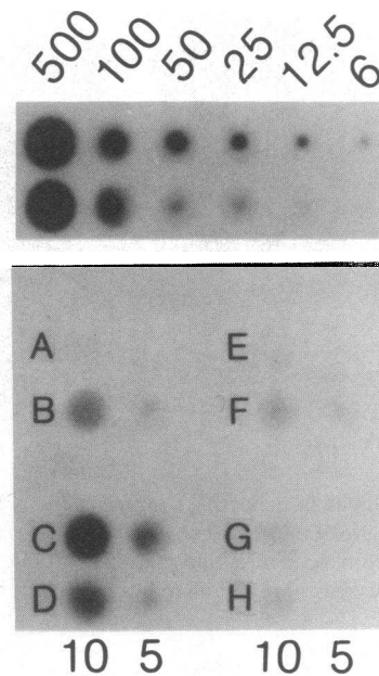
Figure 3. Autoradiograph of dot-blot hybridization for detection of CMV DNA in patients' leukocytes. (Row 1) HCMV DNA in concentrations of 500 to 6 pg using serial dilutions. (Row 2) Similar concentrations of HCMV DNA as in row 1, diluted in 10 µg of human leukocyte DNA obtained from a seronegative healthy donor. (Row 3) Leukocyte DNA from a seronegative healthy donor in concentrations of 10 and 5 µg. (Rows 4–7) Polymorphonuclear and mononuclear leukocyte DNA obtained from four patients with CMV viremia (A.B., C.D., E.F., and G.H.) in concentrations of 10 and 5 µg. The estimated viral genome equivalents per 100 cells for these leukocyte samples are as follows: A = 5, B = 13, C = 47, D = 21, E = 4, F = 6, G = 5, and H = 5.
