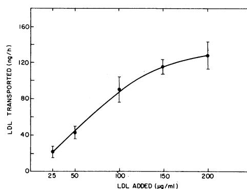
Figure 7. Effect of concentration on LDL transport across RAEC monolayer. ^{125}\text{I} -LDL ( 30,000 \text{ cpm}/\mu\text{g} ) was placed on the apical side of monolayers in the transport units. After 60 min of shaking at 37^\circ\text{C} , LDL transported was determined. Values are mean \pm SD for six monolayers and represent LDL protein transported.
