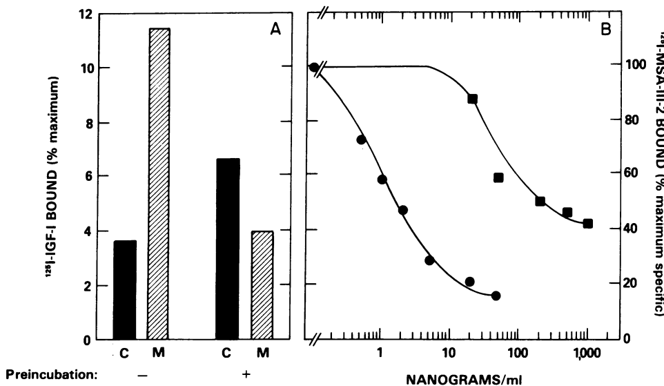
Figure 4. (A) Effect of preincubation of fibroblast monolayers on ^{125}\text{I} -IGF-I binding to cells (C) and media proteins (M). Fibroblast monolayers were grown to confluence in Eagle's MEM-20% fetal calf serum. To one set of cultures (-), ^{125}\text{I} -IGF-I binding to cell monolayers was determined after incubation in HBB for 5 h at 15^\circ\text{C} as described in Methods. At the end of the incubation, the assay media were precipitated with PEG- \gamma -globulin; correction was made for the radioactivity precipitated from tracer and buffer that had not been incubated with cells. Results are expressed as percent total input radioactivity. The solid bars (■) represent the cell-associated ^{125}\text{I} -IGF-I binding, whereas the hatched bars (▨) represent the
