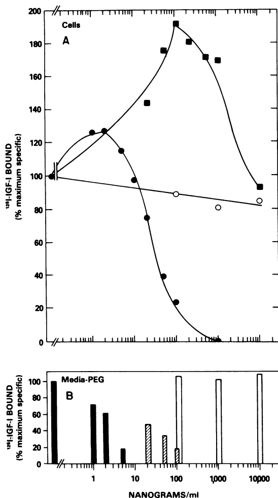
Figure 5. Inhibition of 125 I-IGF-I binding to fibroblast monolayers (A) and media proteins (B) by unlabeled IGF-I (●, ■), A27 insulin -B IGF-I (■, ■), or insulin (○, □). Fibroblasts were grown to confluence in Eagle's MEM-20% fetal calf serum. (A) 125 I-IGF-I binding to fibroblast monolayers was determined in the presence of the indicated peptides. Percent maximum specific binding (3.66% of input radioactivity) is plotted. (B) At the end of the binding incubation, the medium was aspirated, and precipitated with PEG-γ-globulin as described in Methods. Radioactivity specifically precipitated (i.e., after correction for the blank) is plotted as percent of maximum (9.89% of the radioactivity initially incubated with the cell monolayer). No 125 I-IGF-I was specifically precipitated in the presence of ≥10 ng/ml of unlabeled IGF-I or ≥200 ng/ml of A27 insulin -B IGF-I (points not plotted).
