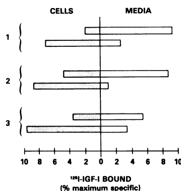
Figure 6. Distribution of 125 I-IGF-I bound to cell monolayers and media proteins for fibroblasts cultivated in serum-containing (S) or serum-free (SF) media. Fibroblasts (S) were plated in Eagle's MEM-20% fetal calf serum (50,000 cells/22-mm well) and grown to confluence (350,000 cells, 72 μg of protein [Bio-Rad assay], per well). Fibroblasts (SF) were plated in Eagle's MEM-0.2% fetal calf serum (150,000 cells/22-mm well) for 48 h, followed by 24 h of incubation in Eagle's MEM-1 mg/ml bovine serum albumin (final concentration 150,000 cells, 40 μg of protein, per well). In experiment 2, cells were plated in 60-mm dishes, resulting in somewhat higher final protein concentrations (300 and 270 μg/well for serum and serum-free conditions, respectively). 125 I-IGF-I binding to cell monolayers (▨) and to media proteins (▤) were determined as described in Fig. 5. The percent maximum specific 125 I-IGF-I bound is shown for three paired experiments.
