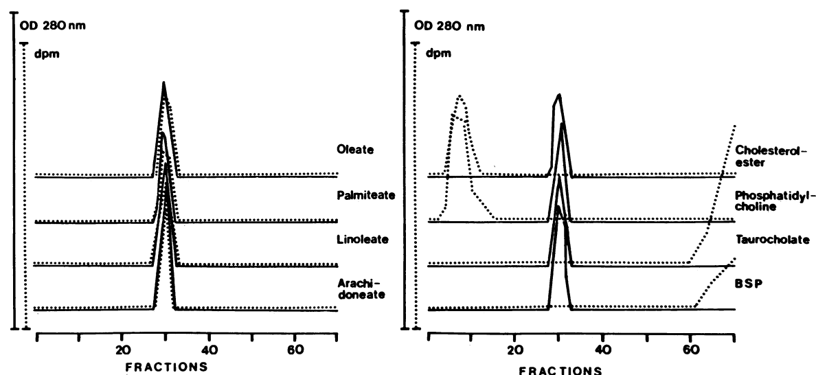
Figure 7. Co-chromatography on Sephadex G-100 of 0.1-mg aliquots of the isolated oleate binding MVM protein with tracer doses of ultrasonically dispersed [ ^{14}\text{C} ]oleate, [ ^{14}\text{C} ]palmitate, [ ^{14}\text{C} ]arachidonate, [ ^{14}\text{C} ]linoleate, [ ^{14}\text{C} ]oleate ester of cholesterol, [ ^{14}\text{C} ]phosphatidylcholine, and [ ^{14}\text{C} ]taurocholate or [ ^{35}\text{S} ]BSP. Only long chain FFA were eluted together with the protein peak. The oleate ester of cholesterol and phosphatidylcholine appeared in the void volume (up to fraction 19), and taurocholate and BSP in the effluent of the column starting at fraction 63. None was associated with protein. See text for experimental details.
