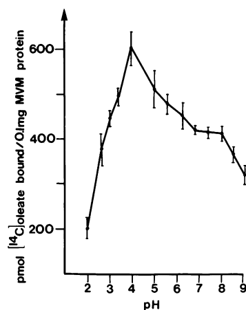
Figure 4. Effect of pH on binding of [ ^{14}\text{C} ]oleate to MVM. 2.272 \mu\text{M} [ ^{14}\text{C} ]oleate free in aqueous solution was incubated with aliquots of 0.1 mg MVM protein in 440 \mu\text{l} citrate-phosphate-borate-/HCl buffer pH 2–9. Values are means \pm SD of three replicate experiments.
