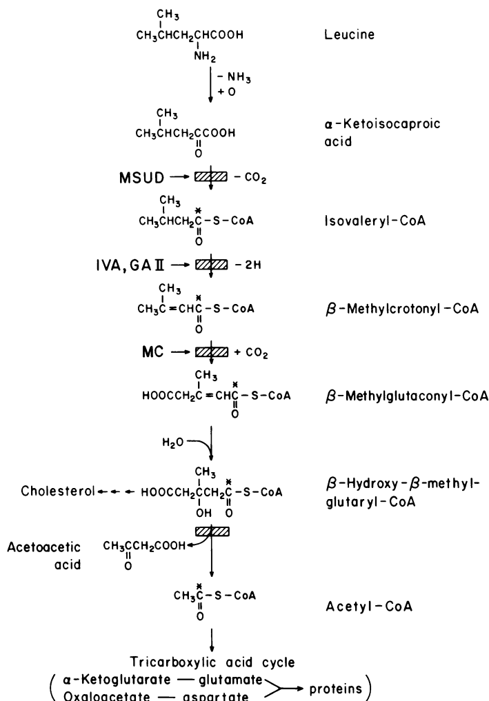
FIGURE 1 The pathway of leucine metabolism and the fate of ^{14}\text{C} from [1\text{-}^{14}\text{C}]\text{isovaleric acid} . The radioactive carbon is marked with an asterisk. The metabolic blocks in MSUD, IVA, and MC are indicated by shaded rectangles.
