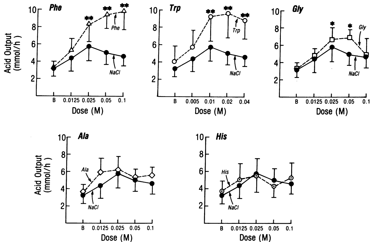
FIGURE 1 Mean ( \pm SE) gastric acid secretory response (mmol/h) to intravenous infusion of graded doses of phenylalanine, tryptophan, glycine, alanine, histidine, and saline (NaCl) control in nine normal subjects. B indicates basal acid secretion. Each dose was infused in 125 ml over 1 h. The responses to 0.025–0.1 M Phe, 0.01–0.04 M Trp, and 0.025 and 0.05 M Gly were significantly different than the NaCl control. ** = P < 0.01 and * = P < 0.05 . The responses to Ala and His were not significantly different than the NaCl control.
