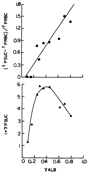
FIGURE 6 Upper panel: plot of the excess sucrose peak transit time ratio (t_{P\text{SUC}} - t_{P\text{RBC}})/t_{P\text{RBC}} vs. \gamma_{\text{ALB}} . The correlation coefficient was 0.876 ( n = 9 , P < 0.001 ). Lower panel: plot of the apparent peak ratio value for sucrose, 1 + \gamma_{P\text{SUC}} , vs. \gamma_{\text{ALB}} .
